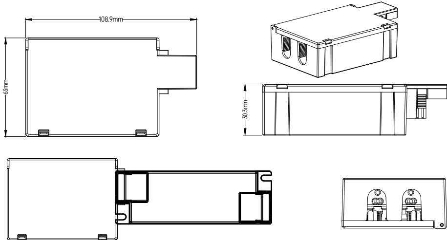
Combined(Side View)
